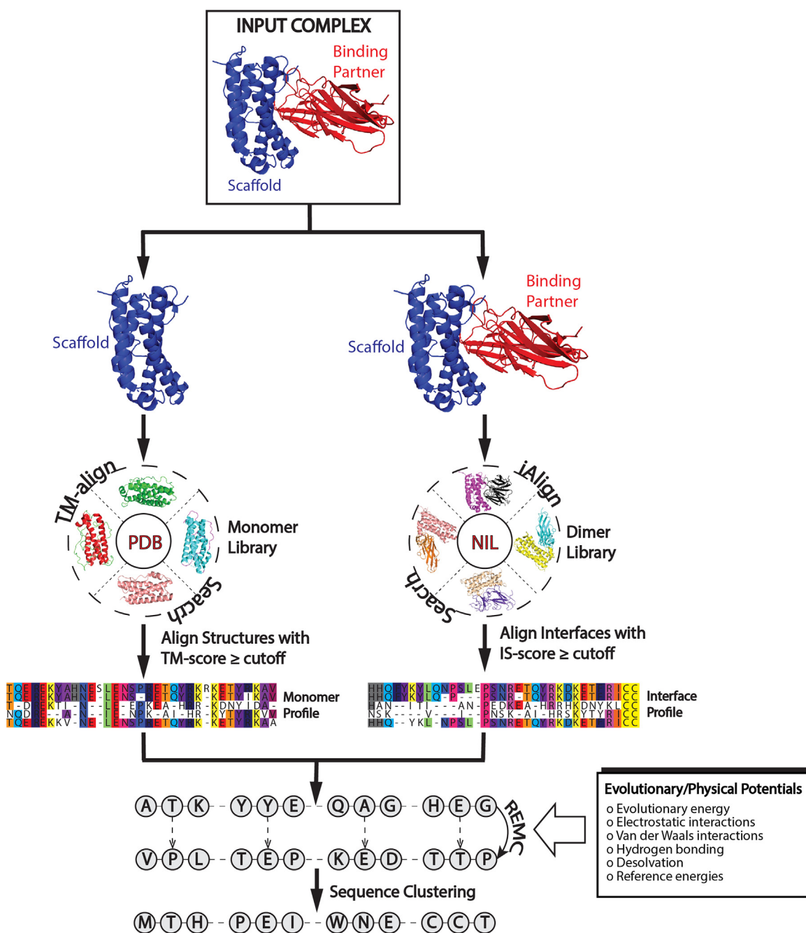
Fig. 1. Flowchart of the EvoDesign pipeline for PPI design. Starting from a given protein complex, similar monomer and interface structures are identified from monomer and dimer structure libraries for the scaffold and protein complex, respectively. Alignments of the structural analogies are used to create evolutionary profiles. These profiles are used as energy terms in conjunction with a physical energy function, EvoEF, to guide the REMC simulation. After clustering the sequence decoys generated during the simulation, the final designs are selected from the lowest free energy sequences in the largest clusters.
