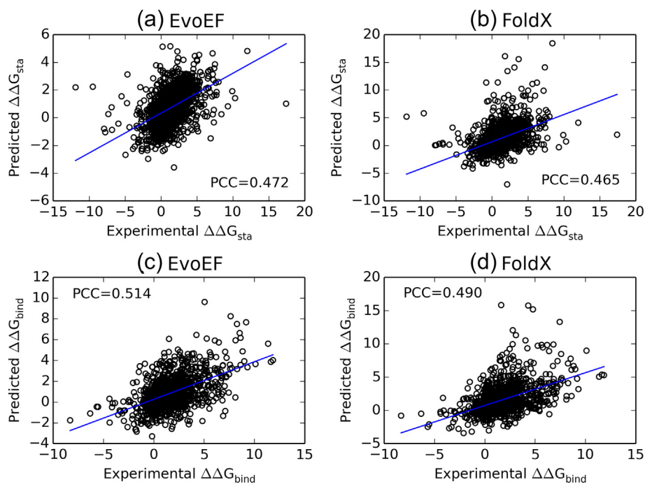
Fig. 2. Correlation between predicted and experimental values for mutation-induced folding stability and binding affinity changes. (a, b) Folding stability changes upon mutation, \Delta\Delta G_{\text{stability}}^{\text{WT}\rightarrow\text{mut}} , for monomer proteins predicted by EvoEF (a) and FoldX (b) versus the experimental data for 1994 test proteins. (c, d) Binding affinity changes upon mutation in the interface of protein–protein complexes, \Delta\Delta G_{\text{binding}}^{\text{WT}\rightarrow\text{mut}} , predicted by EvoEF (c) and FoldX (d) versus the experimental data for 1102 test proteins.
