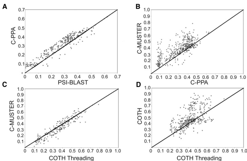
Figure 3. Comparison of TM-Score of the Complex Templates as Identified by Different Threading Methods
