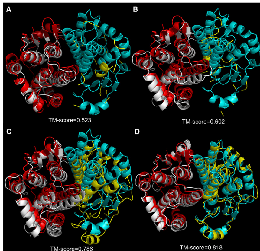
Figure 4. Examples of Improvement over Controls
