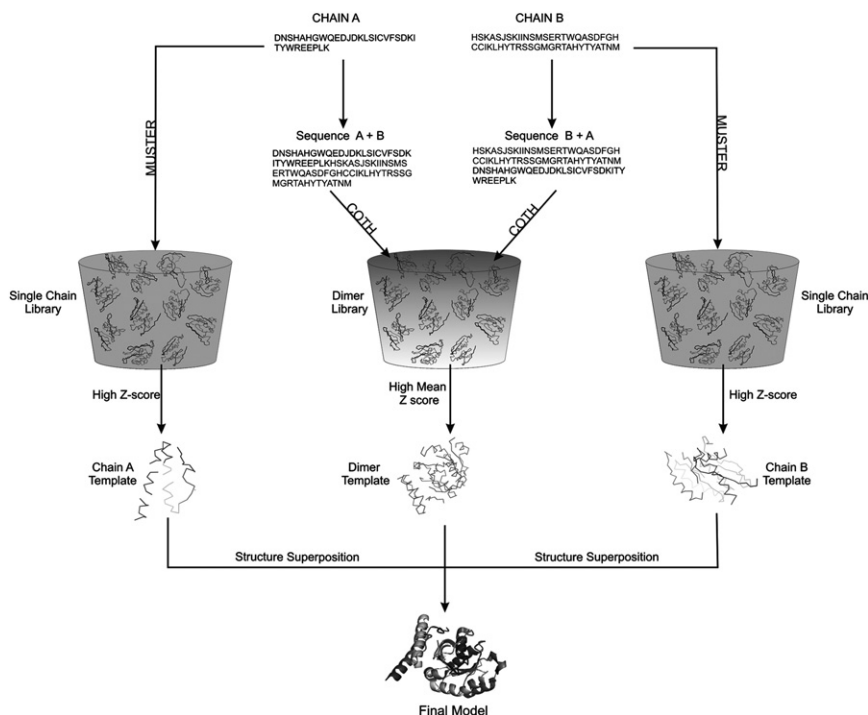
Figure 1. Flowchart of the COTH Algorithm for Protein Complex Template Identification
