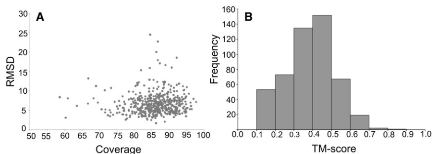
Figure 2. Complex Threading Results by COTH on 500 Nonredundant Test Proteins
