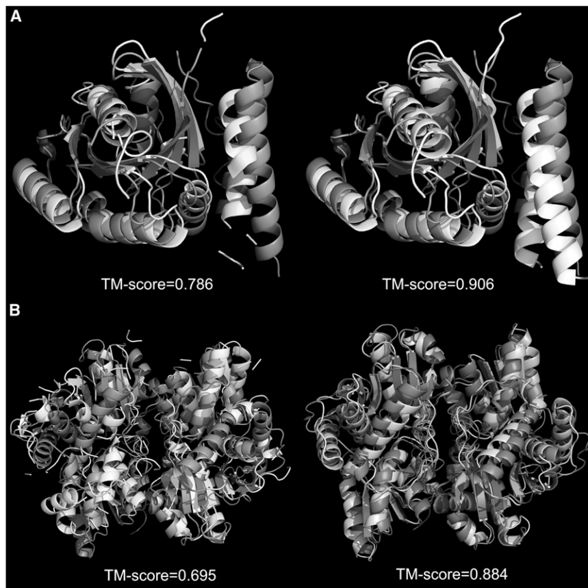
Figure 5. Structure Superposition Improves Template Quality
