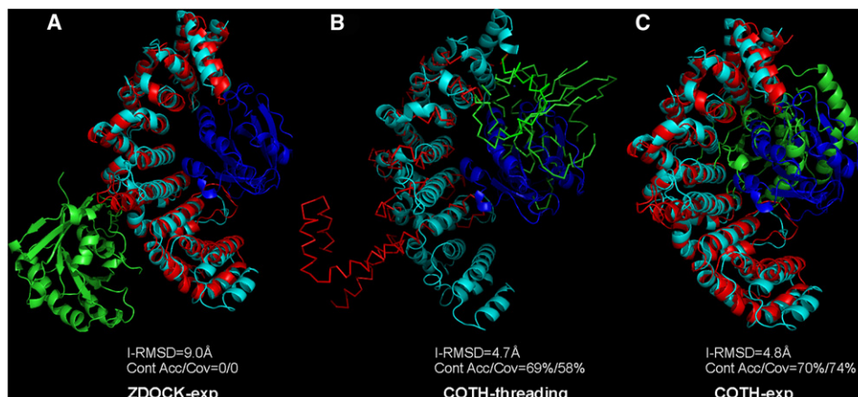
Figure 6. Modeling Result of ZDOCK and COTH on the Ran-Importin \beta Complex
